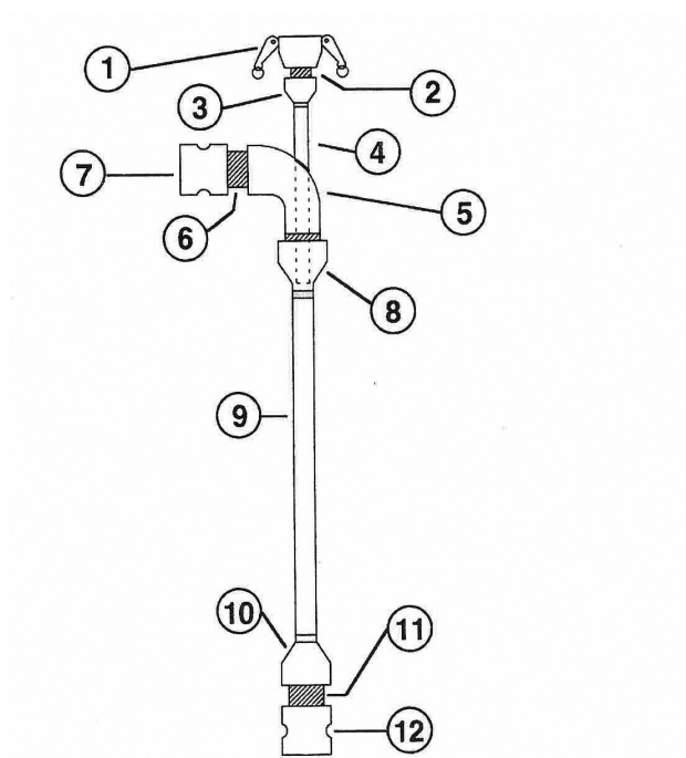
FIGURE SOP 9.4. Rotenone aspirator developed by Utah Division of Wildlife Resources: (1) 2" female cam lock fitting (vacuumed powder enters), (2) 2" x 2" nipple, (3) 2" x 1.25" bell reducer, (4) 1.25" x 12" nipple, (5) 3" 90 degree street elbow, (6) 3" x 3" nipple, (7) 3" male cam lock fitting (lake water enters), (8) 3" x 1.5" bell reducer (powder and water mix), (9) 2" x 48" galvanized pipe, (10) 2" x 3" bell reducer, (11) 3" x 3" nipple, (12) 3" male cam lock fitting (powder-water slurry discharged). Rotenone aspirator was constructed of galvanized pipe (from Thompson et al. 2001).
