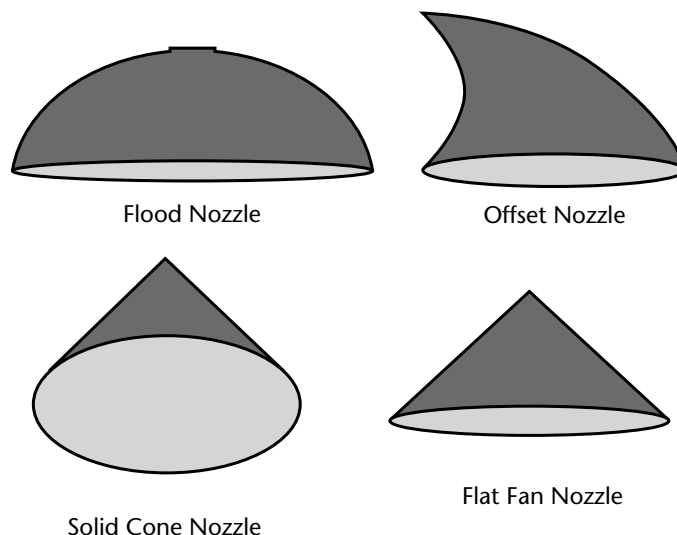
Nozzle Types
