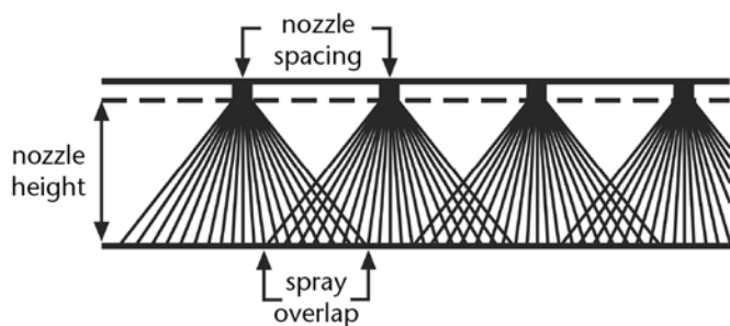
Boom Setup
